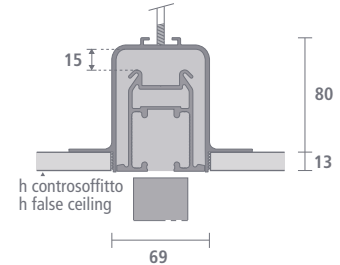
Binario ad incasso Built-in rail
