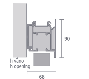
Binario a parete Wall rail
