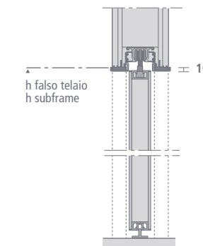
Porta scorrevole per controlelai Scigno® Essential e Eclisse® Syntesis® line Pocket door for systems "Essential" by Scigno® and "Syntesis" line" by Eclisse
