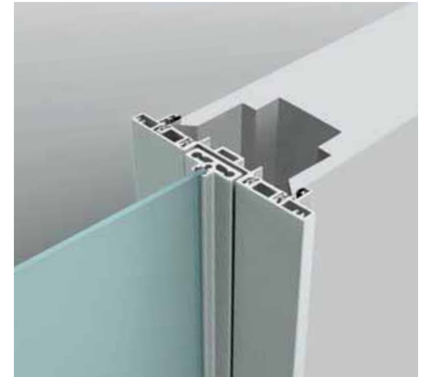
Slim Porta scorrevole per controlelai Scigno® Essential e Eclisse® Syntesis® line Pocket door for systems "Essential" by Scigno® and "Syntesis" line" by Eclisse
