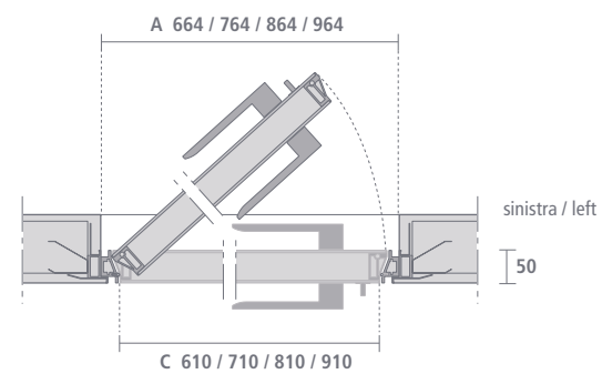
A Luce netta falso telaio Measure of the subframe C Luce netta passaggio Dimensions of the opening
